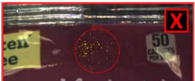
Color pixel count tool confirms the integrity of packaging by identifying pixel values of colors trained in the region of interest.
