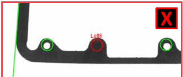
Pixel count tool confirms the presence of 13 separate hole punches within one target by determining pixel value.
